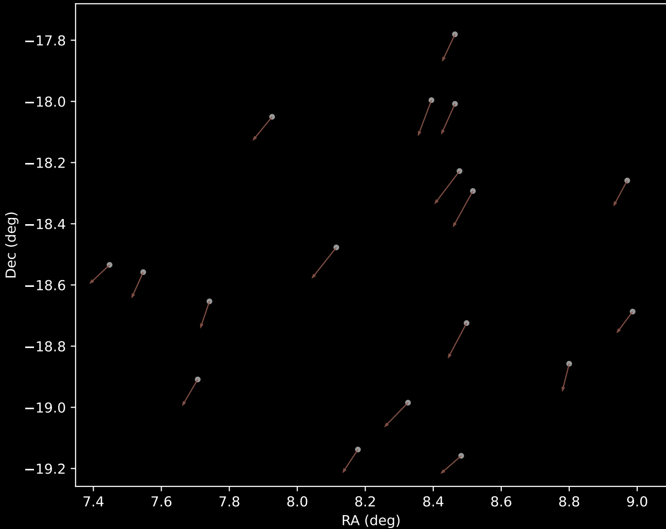
APOGEE DR17 Cluster 10 Proper Motion Vectors (n=18)
