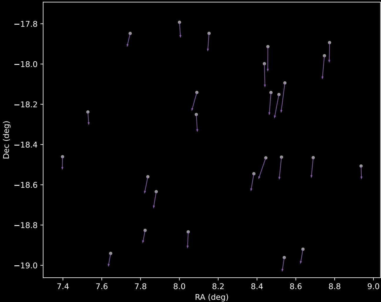
APOGEE DR17 Cluster 8 Proper Motion Vectors (n=26)
