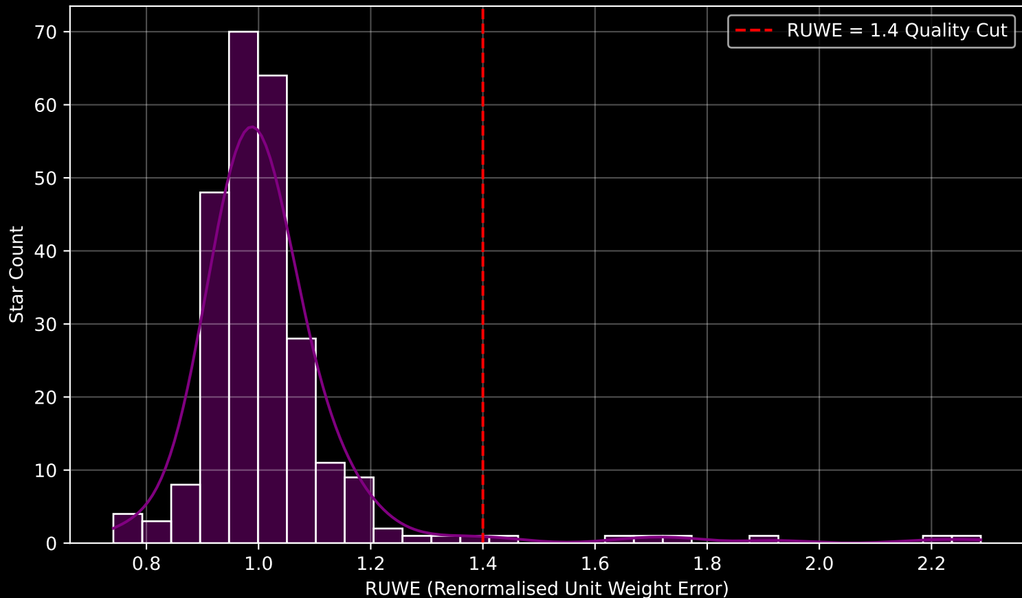
GAPOGEE DR17 Field [010+04] RUWE Distribution (n= 257)
