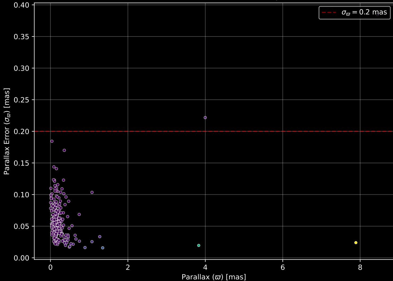
APOGEE DR17 Field: [010+04] Parallax Quality (n= 259)
