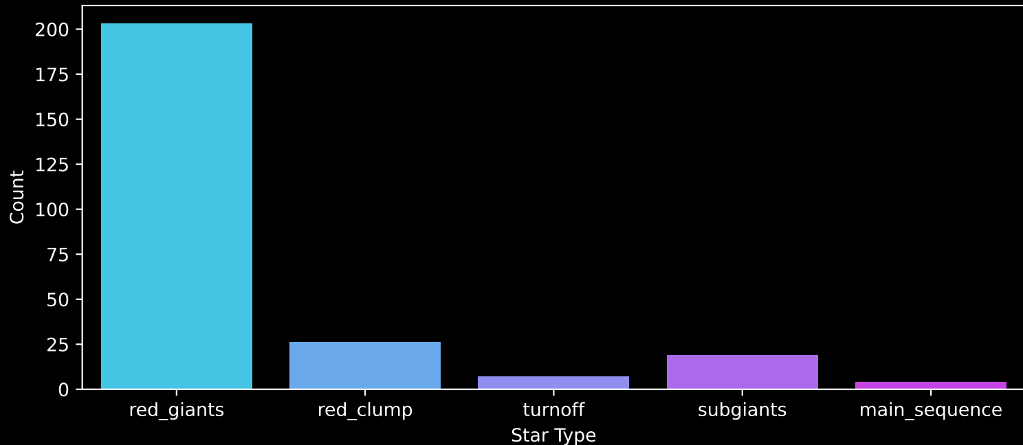
APOGEE DR17 Field: [010+04] Count plot of Star Type
