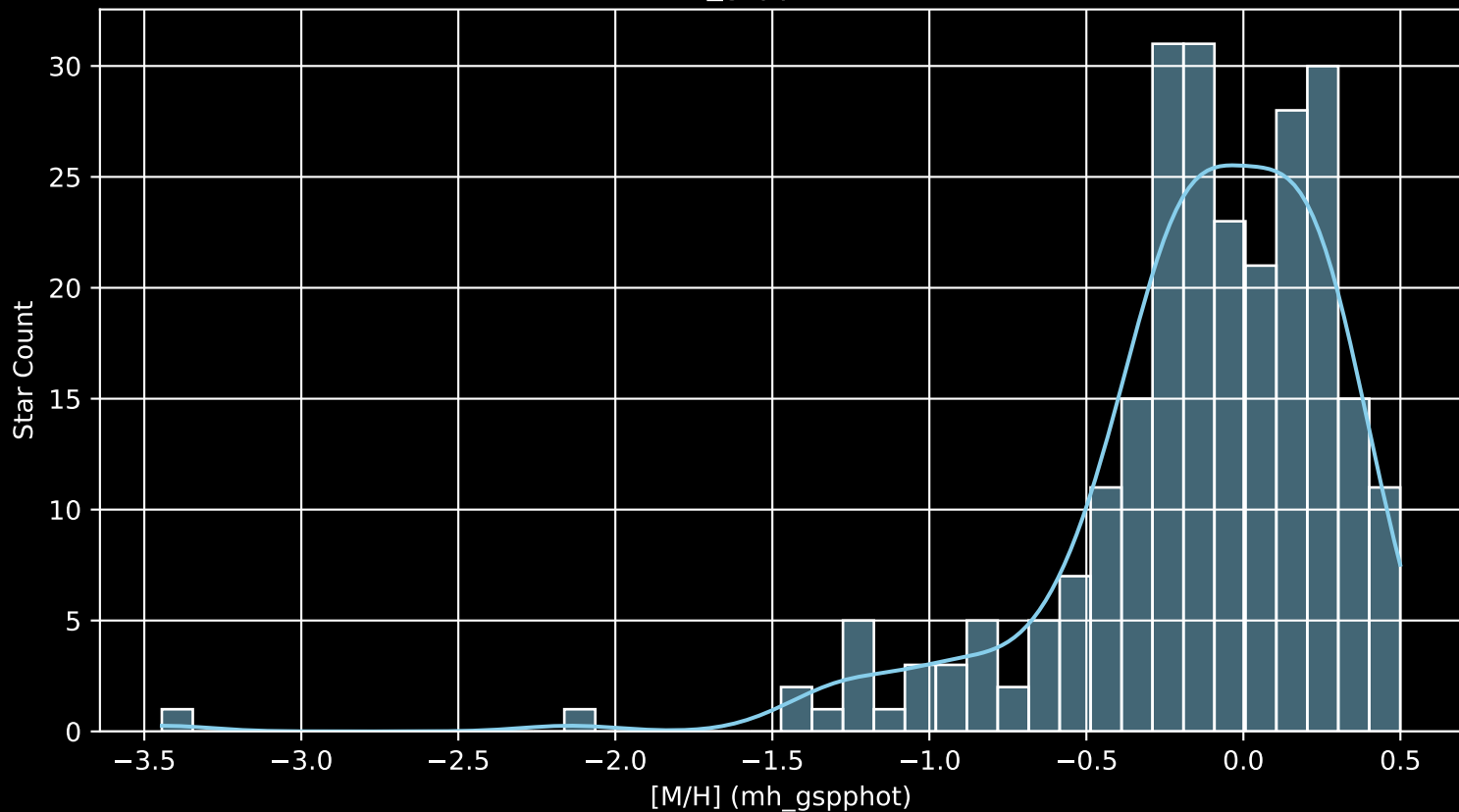
APOGEE DR17 Field: [010+04 [M/H] (mh_gspphot) (n= 252)
