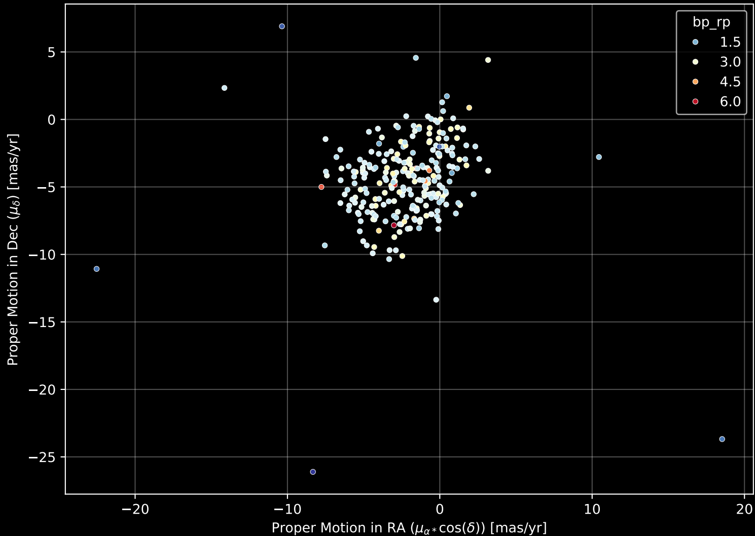
APOGEE DR17 Field: [010+04] Proper Motion Diagram (n= 259)
